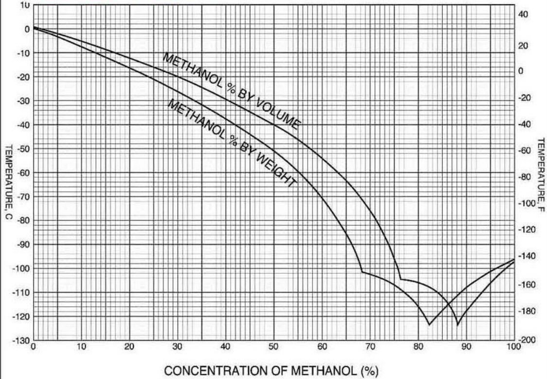
Freezing Point Effect of Methanol - Water Solutions % by weight and by volume
